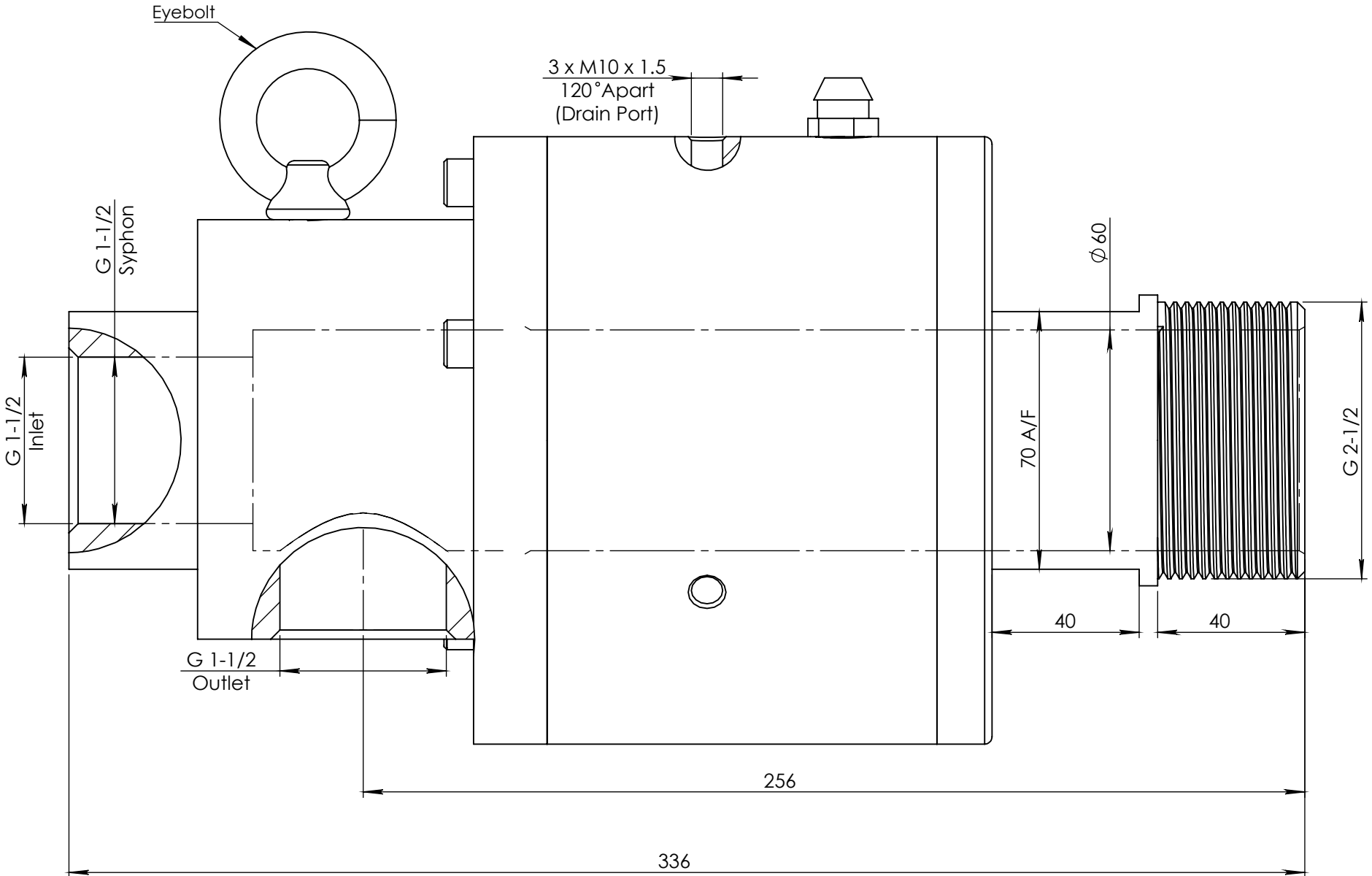
Front View
