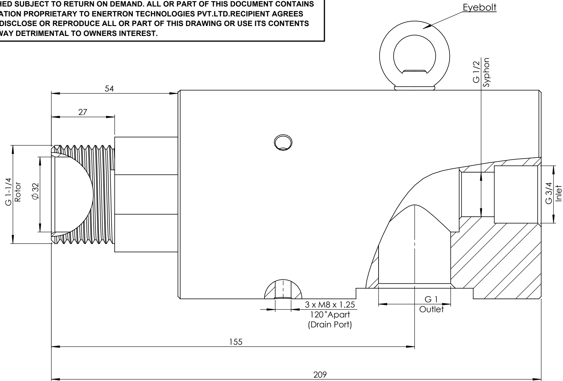
Front View
