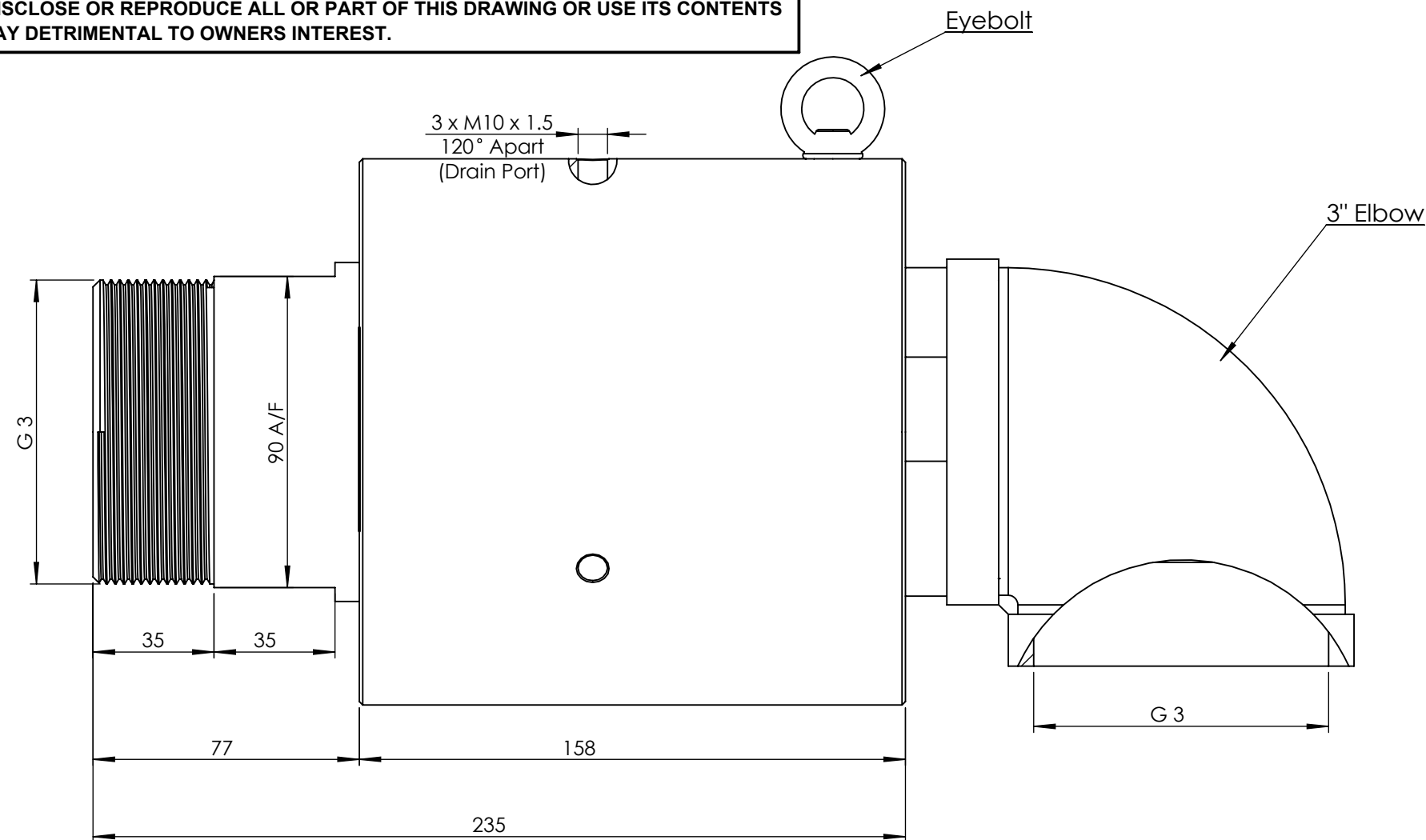
Front View
