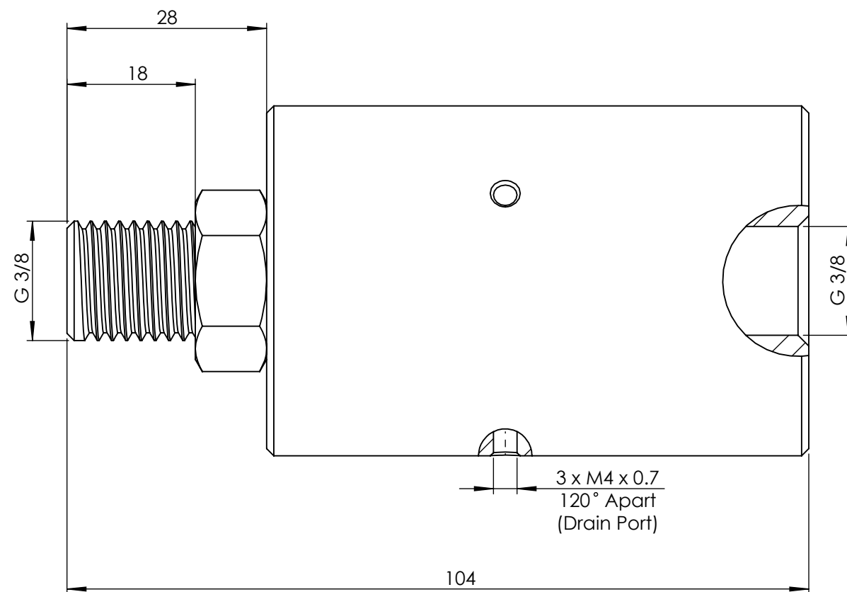
Front View
